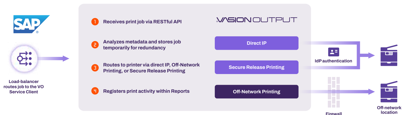
Figure 1. SAP sends the print job to the RESTful API, enabling users to print via Off-Network or Pull Printing. The centralized interface gives administrators control and visibility over printing.
